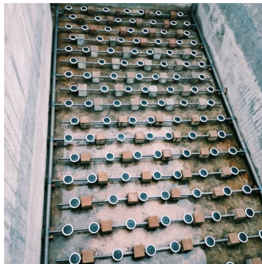
Air Diffusing System at Aeration Tank
