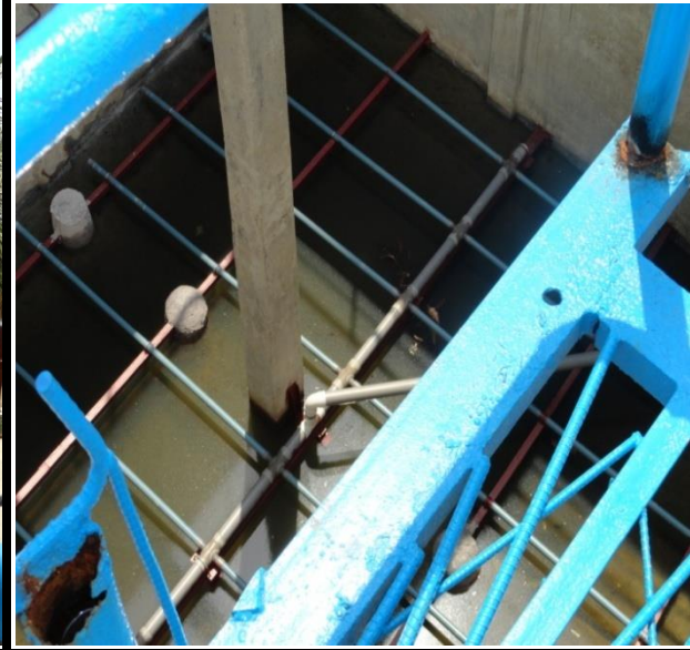
Aeration Tank with air diffusing System
